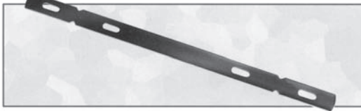
WALL TIES X-FLAT STANDARD 1/4" BREAK BACK-ROLLED EDGES ULTIMATE LOAD (LBS.) 6,000 4" thru 48" stock items. Over 48" built upon request.
